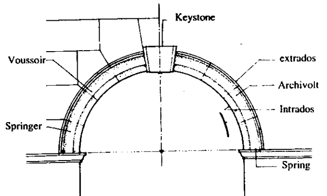
Round Arch
