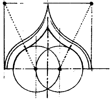
Ogee Arch
