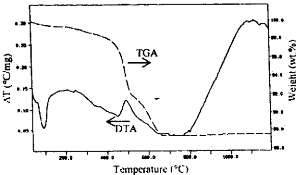
Fig.1 TG-DTA curves for the mixture of \text{Na}_2\text{CO}_3 - \text{K}_2\text{CO}_3 - \text{Nb}_2\text{O}_5 .
