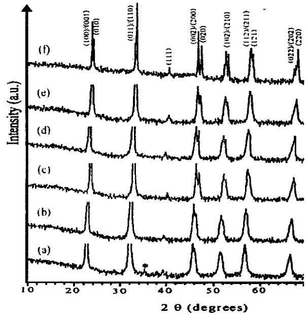
Fig.2 XRD patterns of NKN powder calcined at various conditions; a) 800 °C for 2 h, b) 850 °C for 2 h, c) 900 °C for 2 h, d) 950 °C for 2 h, e) 900 °C for 10 h and f) with an excess of 0.05 mol of starting materials (* = \text{K}_2\text{CO}_3 ).
