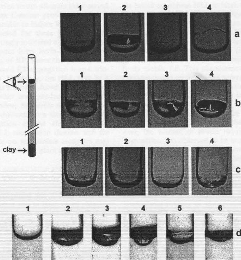
Fig. 6. RP aggregation induced by HLL. (a) Specific staining. After 30 min-incubation of RP with either control buffer (tubes 1 and 3) or 1.8 \mu g of HLL (tubes 2 and 4), the assay mixture (50 \mu l) was stained with either basic Fuchsin (tubes 1 and 2) or Alcian blue (tubes 3 and 4). The RP aggregates were separated by centrifugation and viewed with a light microscope. (b) Time course of HLL-induced RP aggregation. After the assay mixtures (50 \mu l, each) containing RP and HLL (1.8 \mu g) were incubated for 5, 10, 20 and 40 min as in tubes 1, 2, 3 and 4, respectively, and stained with Fuchsin. The amounts of RP aggregates obtained after centrifugation were compared. (c) Effect of various proteins other than HLL on RP aggregation. After 30 min-incubation of the RP with either control buffer (tube 1), 10 \mu g of BSA (tube 2), 2.5 \mu g of fetuin (tube 3), or 8 \mu g of C-serum protein, the assay mixture was stained, separated by centrifuged and the amount RP aggregates were compared. (d) HLL induced aggregation of non- Hevea RP. HLL (1.8 \mu g) was incubated with either isotonic buffer (tube 1) or RP suspension prepared from the latex of Calotropis gigantea (tube 2); Euphorbia mili DesMoulin (tube 3); Ficus elastica Roxb (tube 4); Plumeria rubra Linn. (tube 5); Argyrea capitiformis (tube 6) for 30 min. The mixtures were stained and the RP aggregates were separated and visualized.
