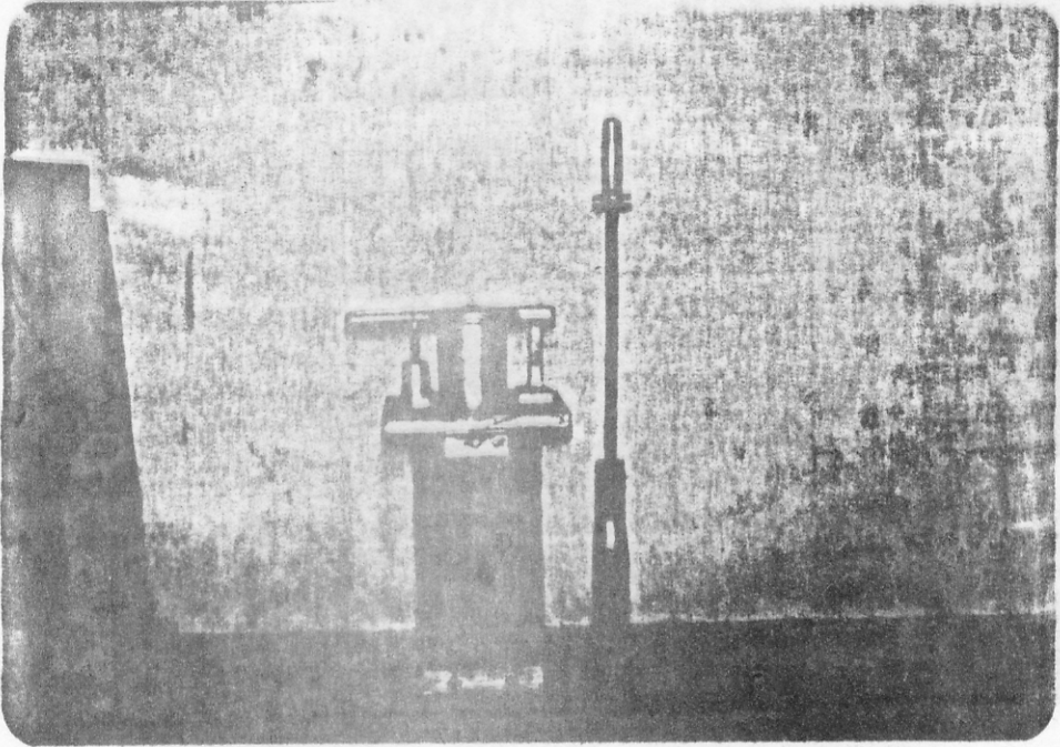
Pedestal hammer and mold holder for preparing specimen
