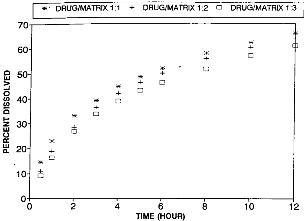
Figure 1 : Theophylline dissolution profile in simulated gastric fluid pH 1.2
