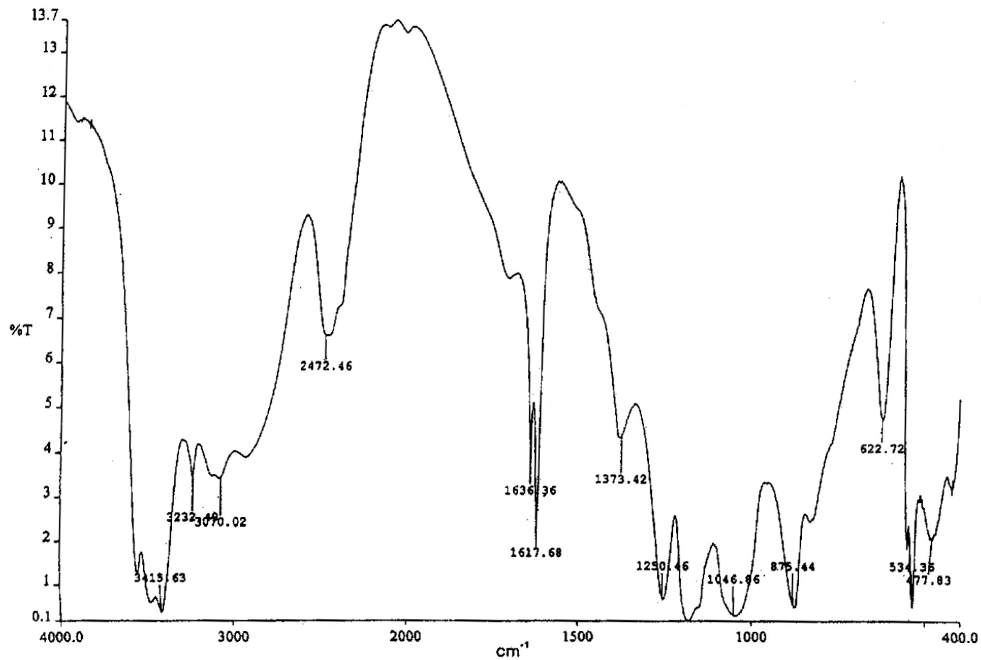
(A) Infrared spectrum of SephadexG-75 fraction
