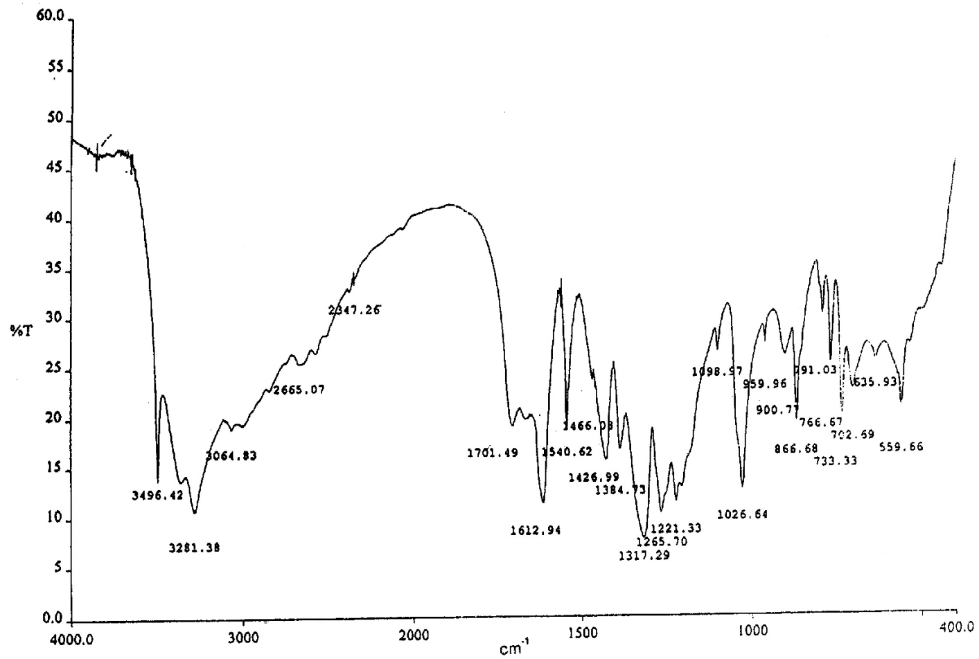
(C) Infrared spectrum of Gallic acid
