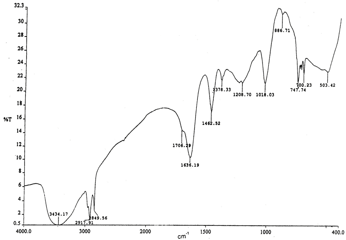
(B) Infrared spectrum of hydrolyzed SephadexG-75 fraction
