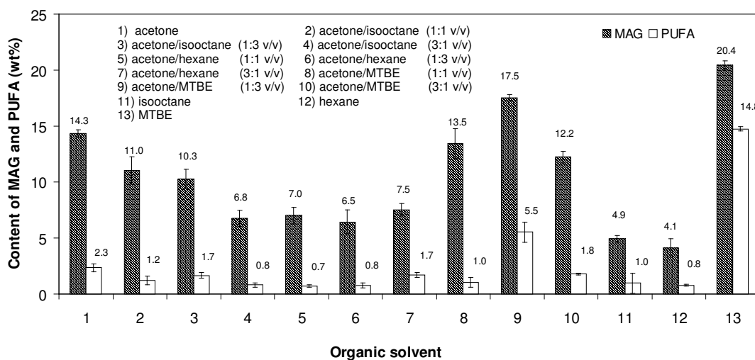
Figure 8. Screening of organic solvents on MAG production with IM-AK. The reaction mixture contained 20 ml of 30 %w/v tuna oil in organic solvents and 1.78 g glycerol with 4 wt% water. The amount of IM-AK used was 0.6 g (0.46 U/mg). The reaction was carried out at 300 rpm and 45°C for 24 h.
