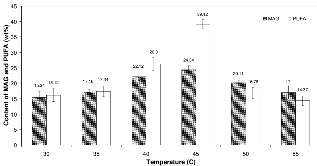
Figure 12. Effect of temperature on MAG production. The reaction mixture contained 20 ml of 10 %w/v of tuna oil in MTBE and 1.78 g glycerol with 4 wt% water. The reaction was carried out at 300 rpm for 24 h.
