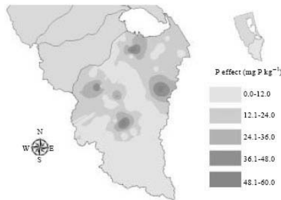
Fig. 7: Phosphorus amounts (mg P kg -1 ) in U-Tapao and Eastern Coast Sub Basin 4 Sub-watershed obtained using AnnAGNPS model
