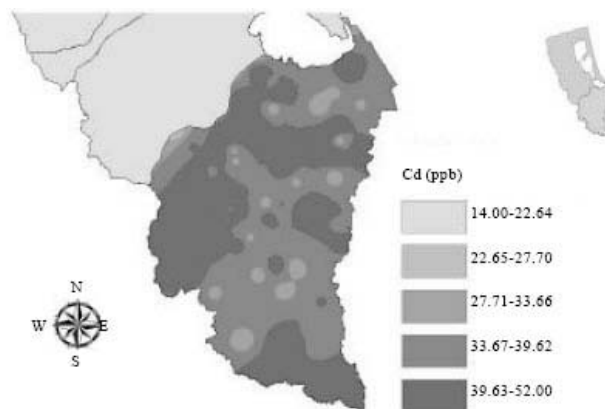
Fig. 8: Cadmium amounts (ppb) in U-Tapao and Eastern Coast Sub Basin 4 Sub-watershed obtained using TRES model
