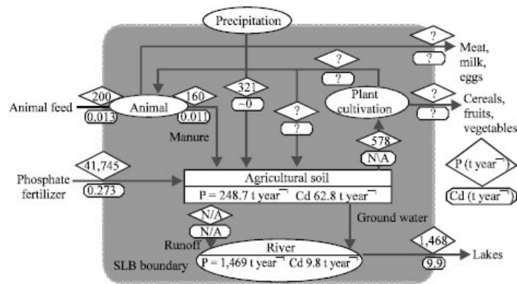
Fig. 6: SFA of phosphorus (diamond) and cadmium (rounded rectangle) in SLB ( \text{t year}^{-1} )
