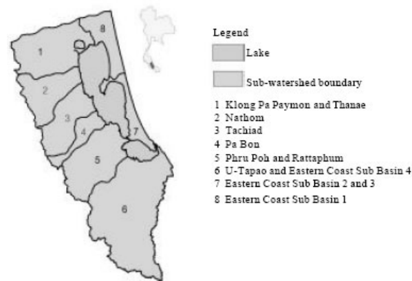
Fig. 2: Sub-watersheds of the Songkhla Lake Basin
