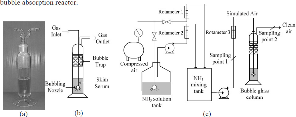
Figure 1. Bubble glass absorption reactor picture (a), diagram of the bubble reactor (b), and schematic diagram of \text{NH}_3 contaminated air treatment system by bubble reactor (c).
