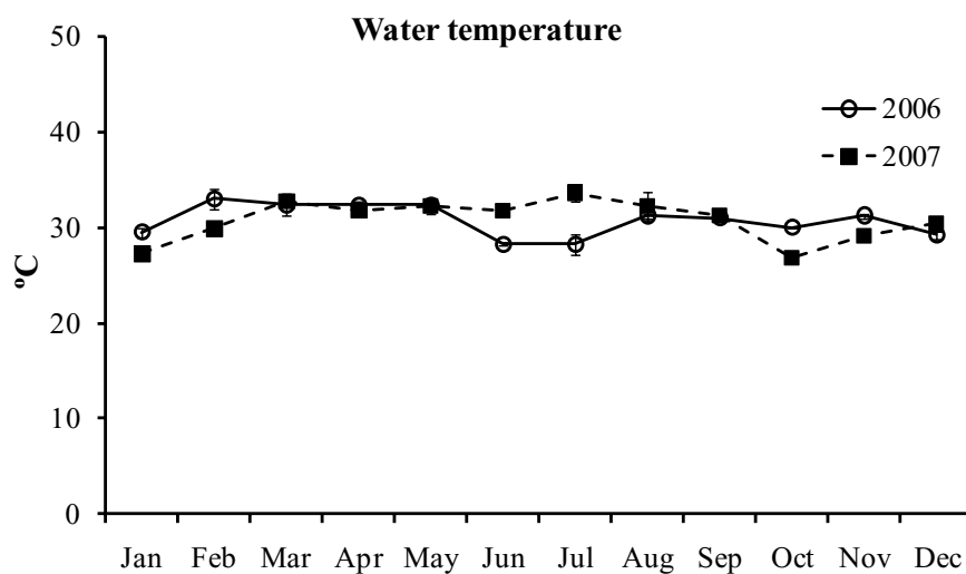
Figure 12. Seasonal changes in water temperature from January 2006 to December 2007. The error bars are standard error. (n=144)
