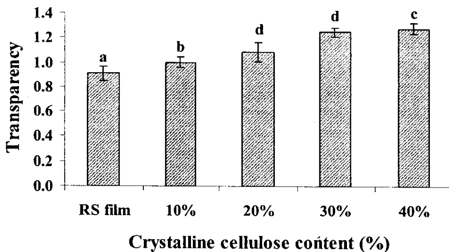
Figure 40. Effect of content of CC on transparency of RS films. Mean values with different letter are significantly different ( p < 0.05 ).
