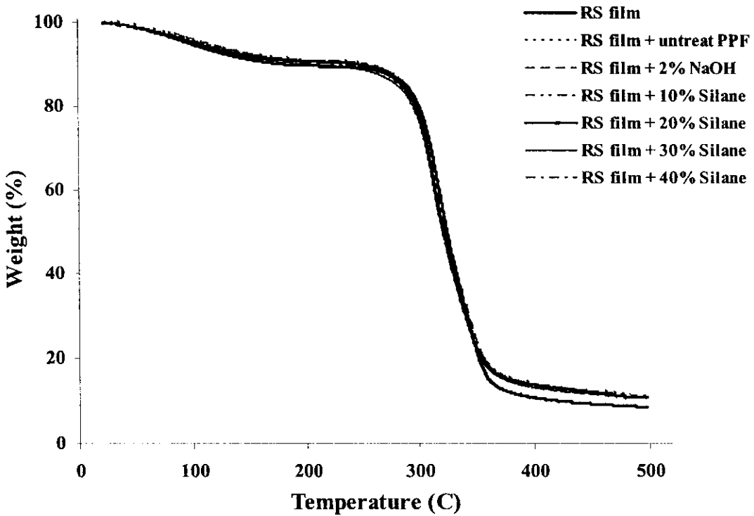
Figure 29. TGA thermograms of RS films, RS film reinforced with untreated PPF and treated PPF (30% of starch).
