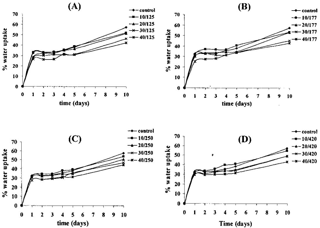
Figure 12. Effect of size and content of PPF at (A) 125 \mu\text{m} , (B) 177 \mu\text{m} , (C) 250 \mu\text{m} and (D) 420 \mu\text{m} on water uptake of RS films.
