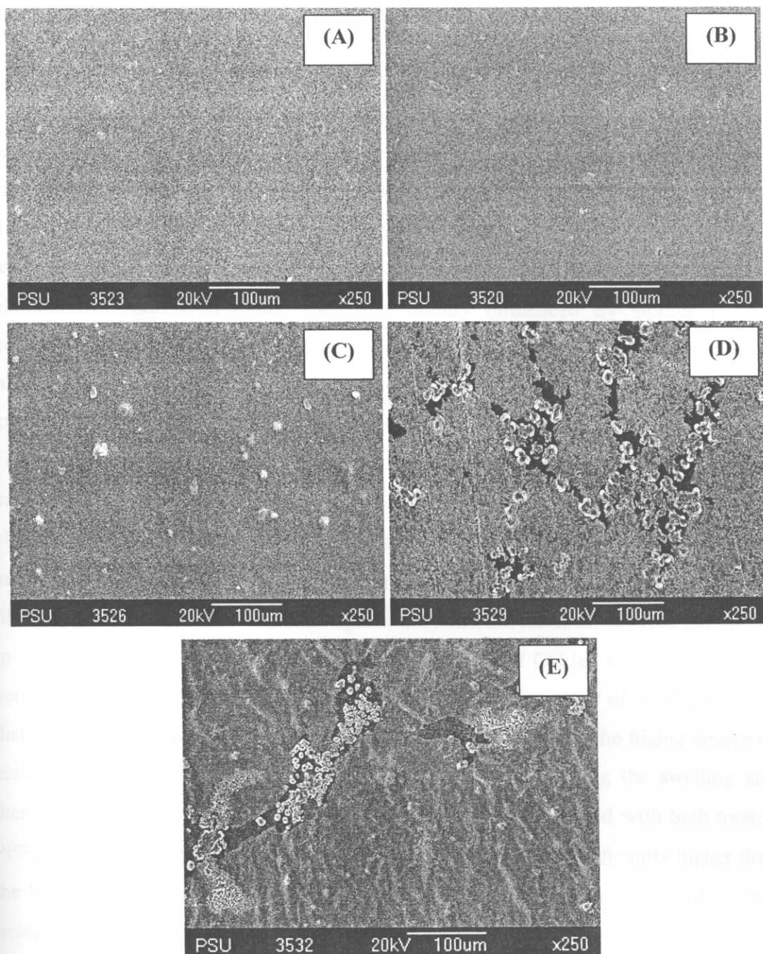
Figure 44. Scanning electron micrograph (SEM) ( \times 250 ) of the RS films reinforced with (A) 0%, (B) 10%, (C) 20%, (D) 30% and (E) 40% of CC fillers.
