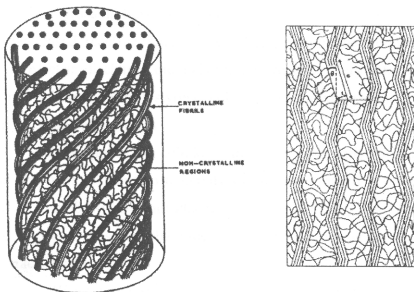
Figure 7. Crystalline and amorphous structure of the fiber
