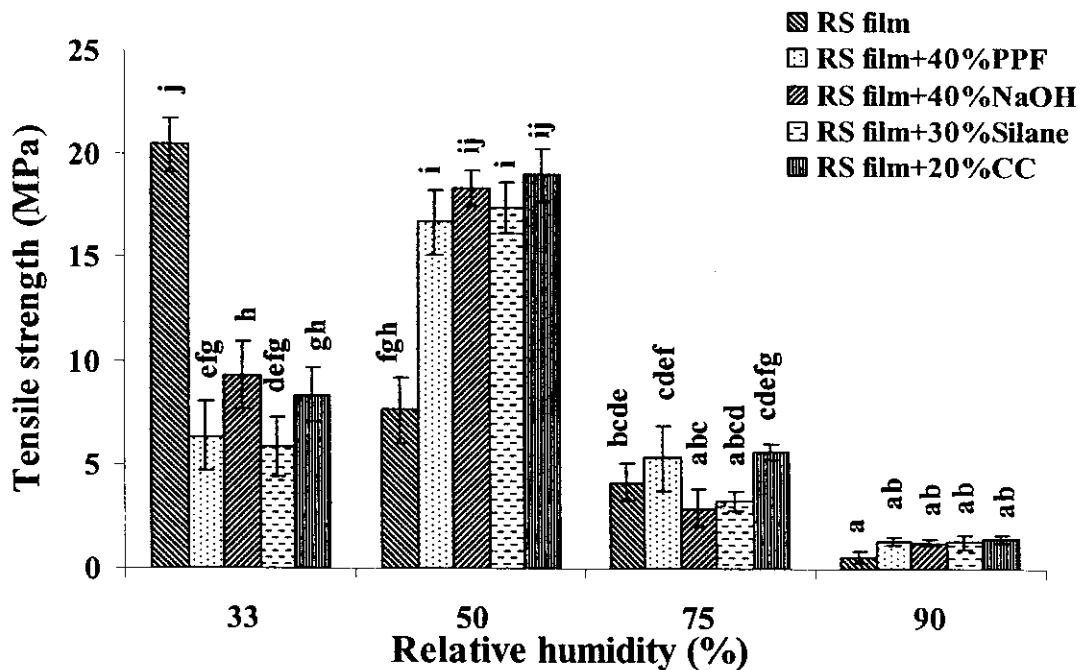
Figure 46. The tensile strength of the RS film and RS films reinforced with different fillers conditioned at different relative humidity. Mean values with different letter are significantly different ( p < 0.05 ).
