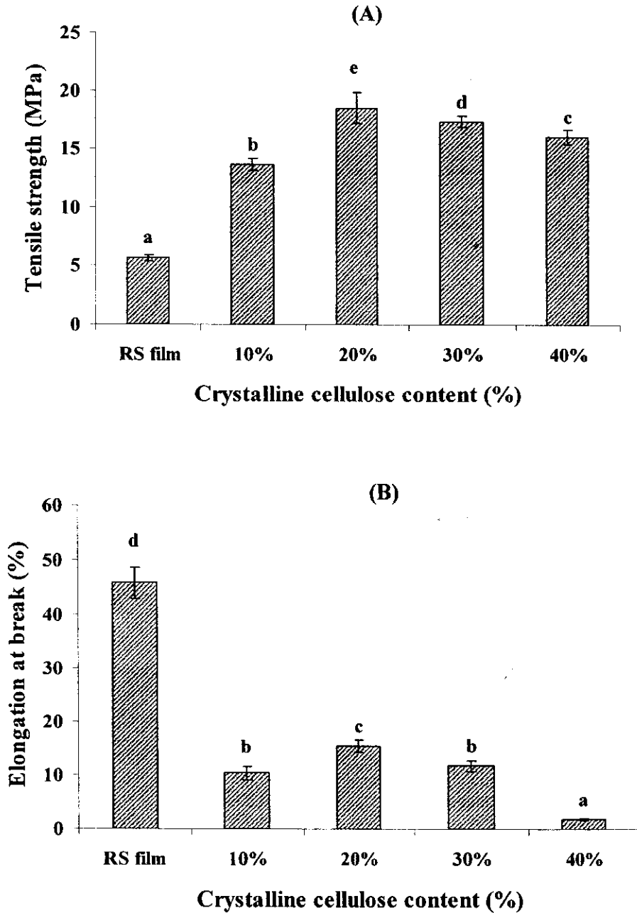
Figure 35. Effect of content of crystalline cellulose (CC) on tensile strength (A) and elongation at break (B) of RS films. Mean values with different letter are significantly different ( p < 0.05 )
