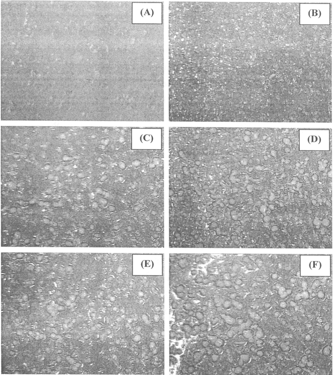
Figure 32. Surface ( \times 10 ) of RS films reinforced with (A) untreated, (B) 2% NaOH, (C) 10% Silane, (D) 20% Silane, (E) 30% Silane and (F) 40% Silane PPF at 30% PPF fillers.
