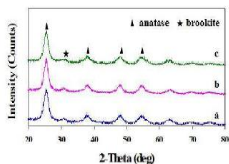
Fig.2 XRD patterns of synthesized powders calcined at 100^\circ\text{C} for 24 h (a) \text{TiO}_2 , (b) 0.5\text{mol}\%\text{Fe}^{3+}/\text{TiO}_2 (c) 5\text{mol}\%\text{N}/\text{TiO}_2
