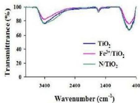
Fig.3 FT-IR spectra of powders synthesized at 100^\circ\text{C} for 24 h (a) \text{TiO}_2 , (b) 0.5\text{mol}\%\text{Fe}^{3+}/\text{TiO}_2 (c) 5\text{mol}\%\text{N}/\text{TiO}_2
