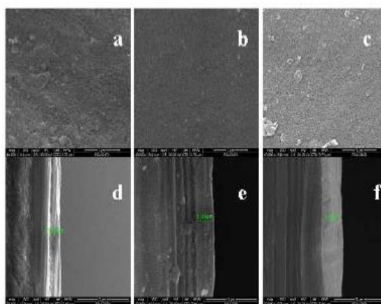
Fig. 1 SEM images of thin film surfaces and cross-sections of (a), (d) \text{TiO}_2 , (b), (e) 0.5\text{mol}\%\text{Fe}^{3+}/\text{TiO}_2 and (c), (f) 5\text{mol}\%\text{N}/\text{TiO}_2
