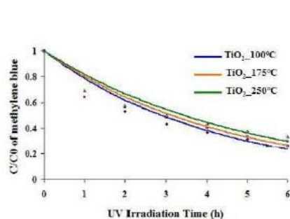
Fig.4 Photocatalytic activity of TiO 2 thin films synthesized at various temperatures.
